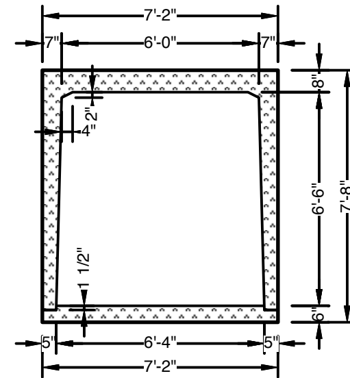
SECTION VIEW Showing Keyed Floor Slab
