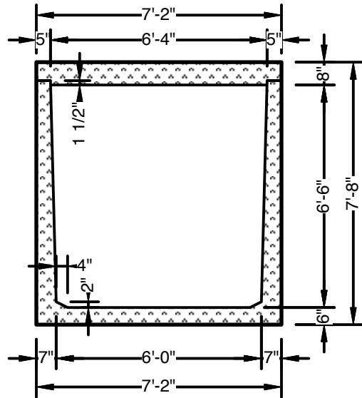
SECTION VIEW Showing Removable Roof
