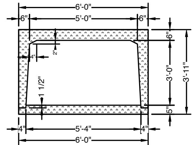
SECTION VIEW Showing Keyed Floor Slab
