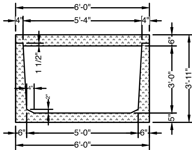
SECTION VIEW Showing Removable Roof
