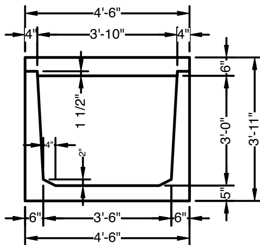
SECTION VIEW Showing Removable Roof
