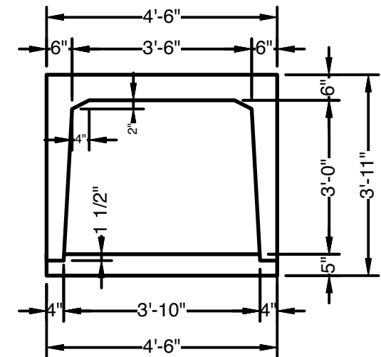
SECTION VIEW Showing Keyed Floor Slab
