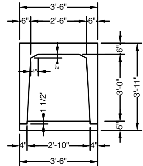
SECTION VIEW Showing Keyed Floor Slab
