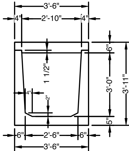
SECTION VIEW Showing Removable Roof
