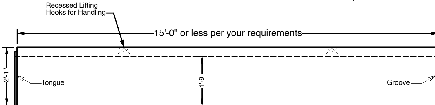
SIDE VIEW
