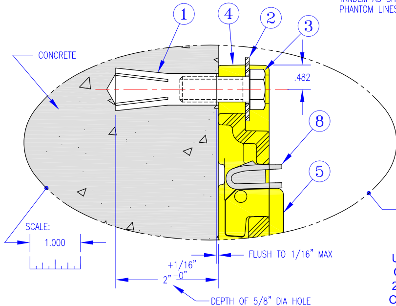
DETAIL No.1
