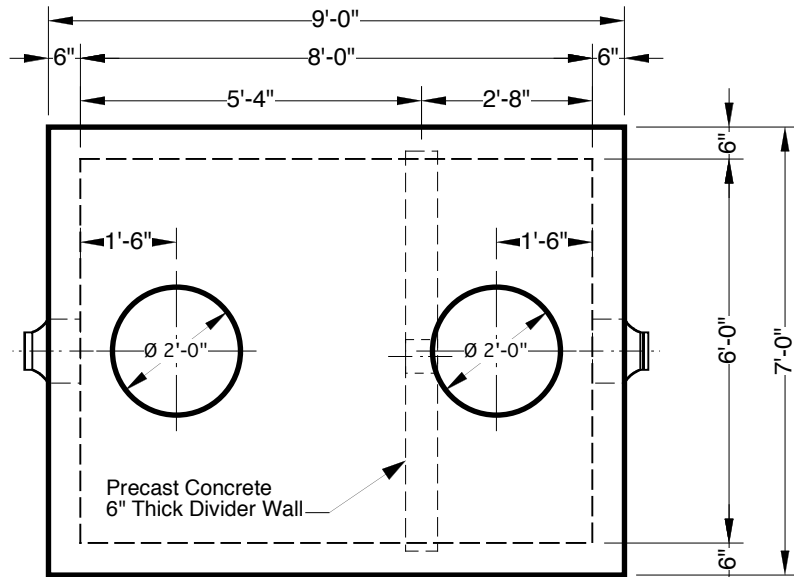
PLAN VIEW (without frames & covers)
