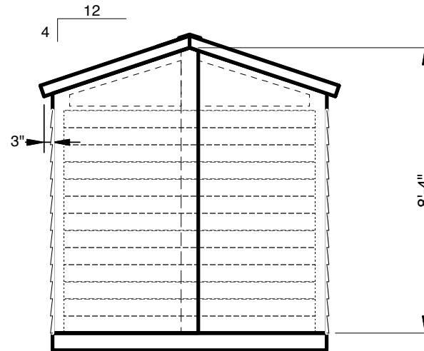
END VIEW
